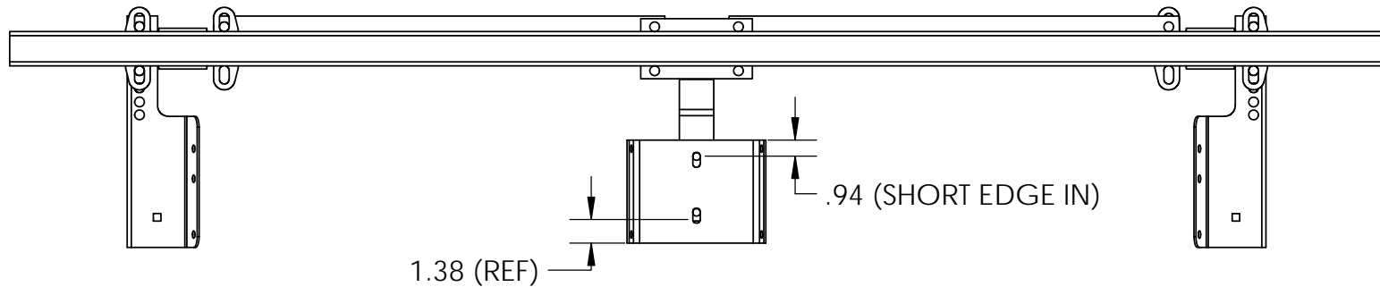
2" WIDE FRAME ON ALL PONTOON TRAILERS
