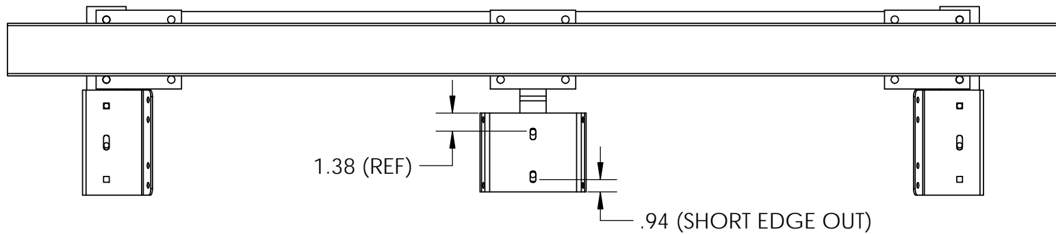
4" WIDE FRAME ON ALL PONTOON TRAILERS
