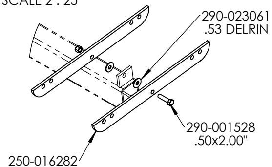
DETAIL A SCALE 2 : 25
