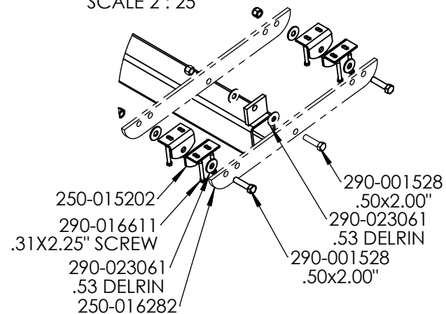
DETAIL A SCALE 2 : 25
