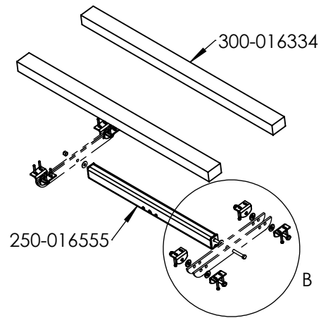
DETAIL B SCALE 2 : 25
