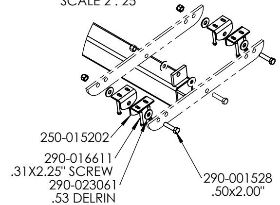
DETAIL A SCALE 2 : 25
