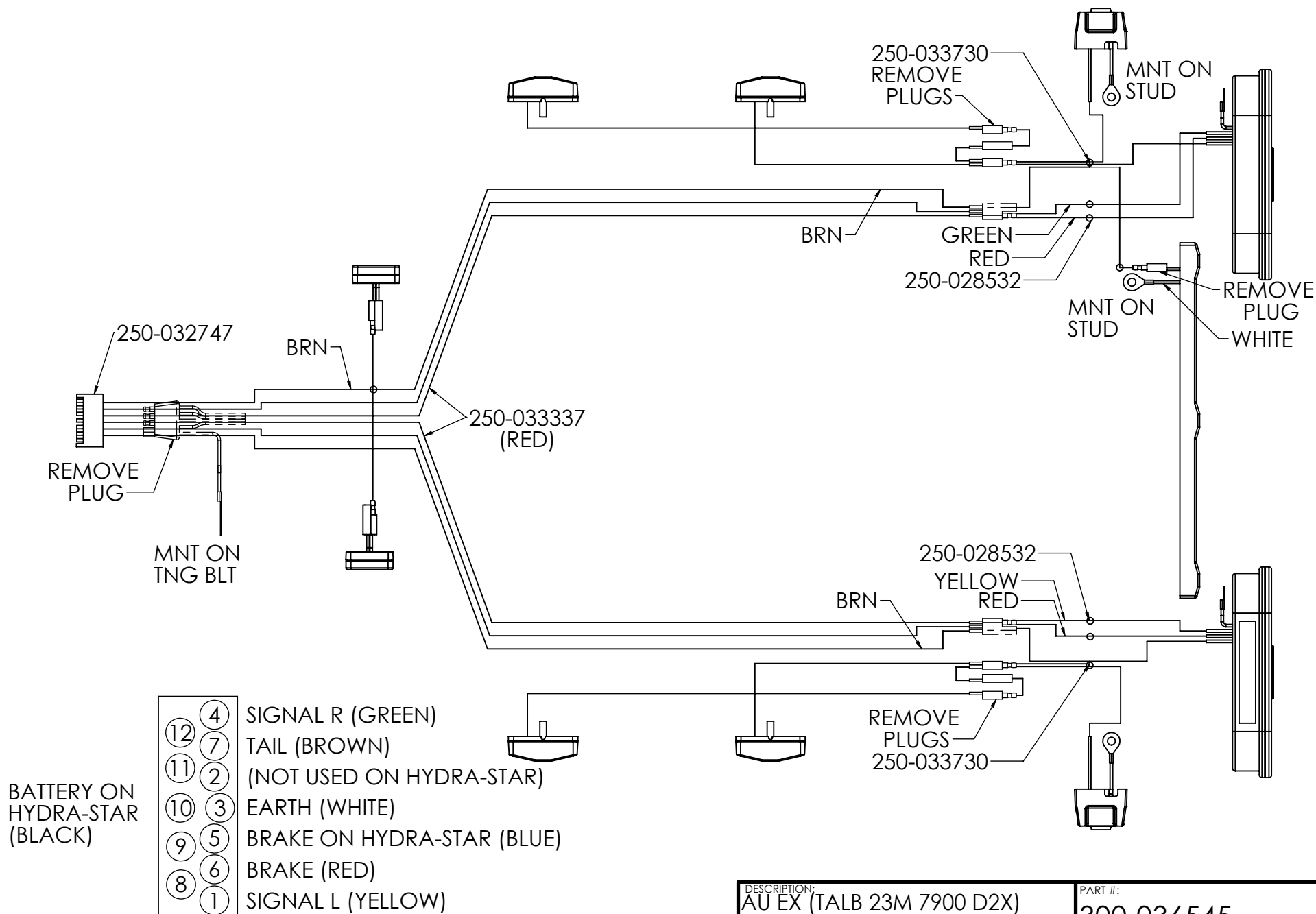
12 PIN HYDRA-STAR PLUG WIRING DETAIL
