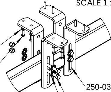
DETAIL B SCALE 1 : 10
